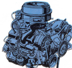
5.0 Liter V8 (305 Cu. In.) . Features a staged 4-barrel carburetor and Electronic Spark Control. (ESC not available in Calif.)
